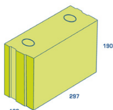
BIA ECO-12/19
