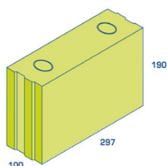
BIA ECO-10/19
